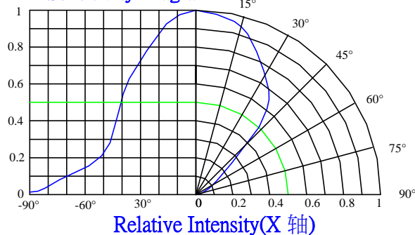
Sensitivity Diagram
