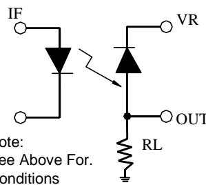
Switching Time Test Circuit
