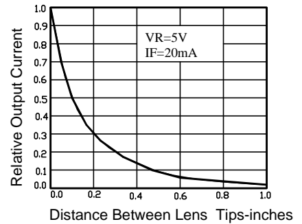
Coupling Characteristics
