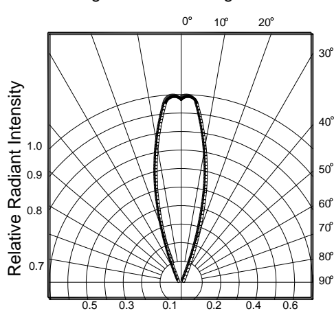
Fig.6 Radiation Diagram
