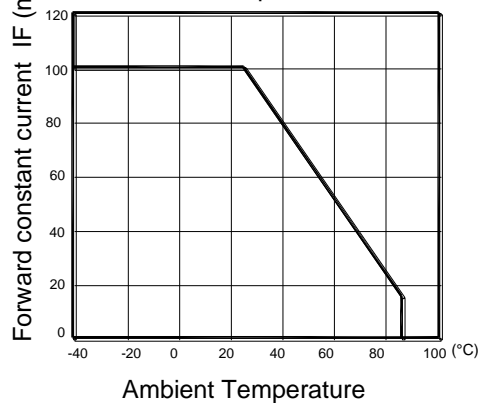
Fig.2 Forward constant current I_F (mA) Vs Ambient Temperature
