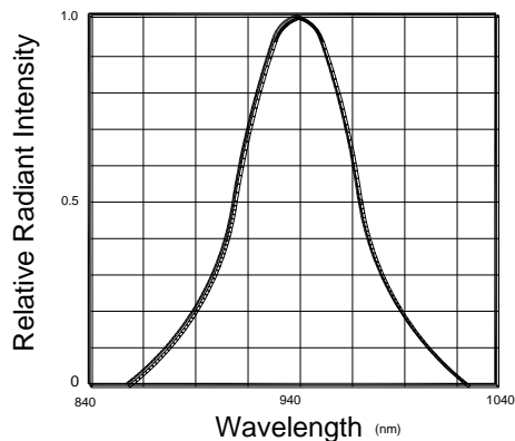
Fig.1 Spectral Distribution
