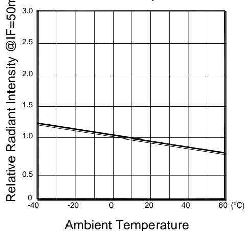
Fig.4 Relative Radiant Intensity Vs Ambient Temperature @ I_F=50\text{mA}
