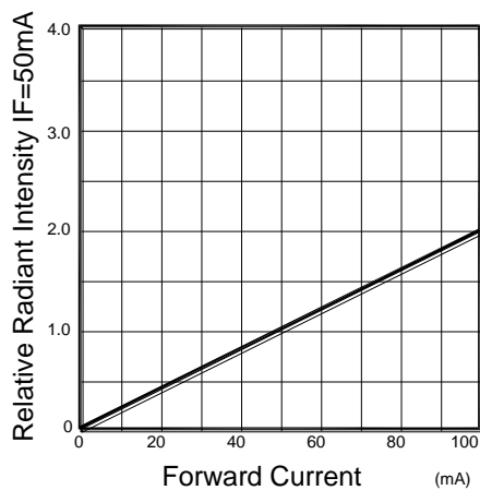
Fig.5 Relative Radiant Intensity Vs Forward Current @ I_F=50\text{mA}
